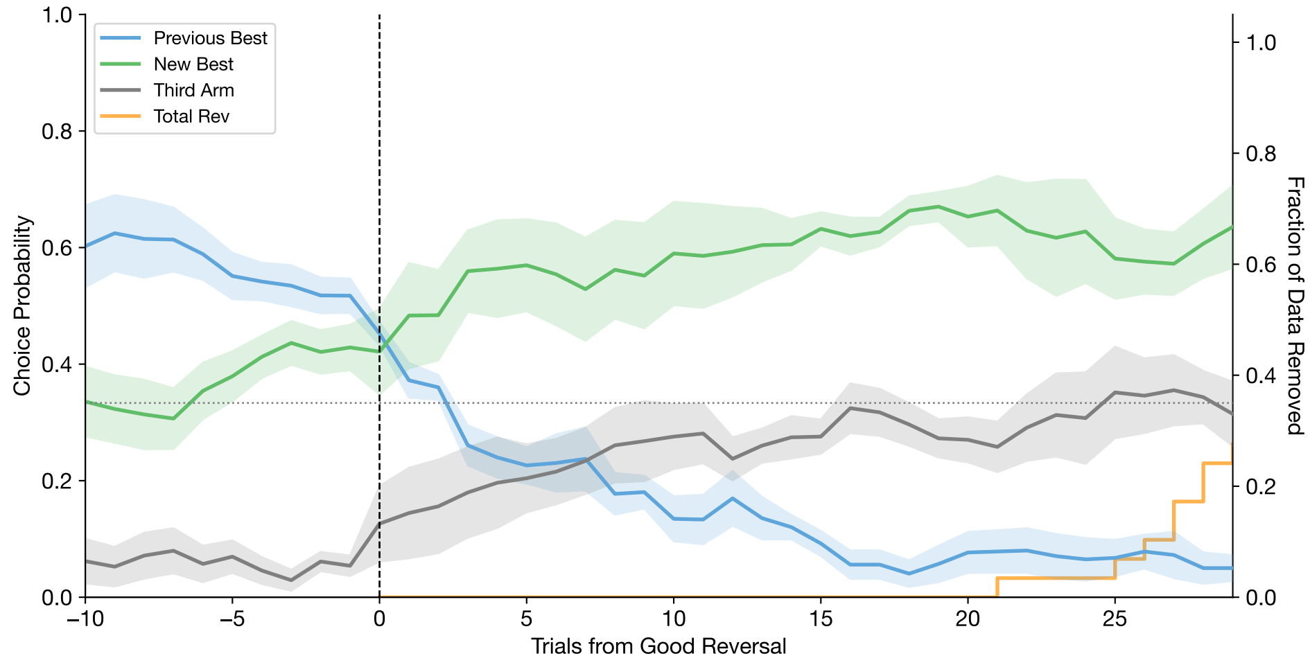
Good Reversal-Aligned Choices (mean \pm se across subjects | n=5 subjects, n=29 reversals)
